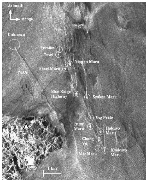
Figure 5. TerraSAR-X SpotLight HH amplitude image used for vessel detection and classification (20.09.2012).
